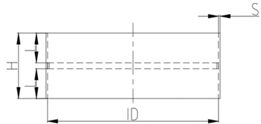
AGRU DOUBLE SOCKET
