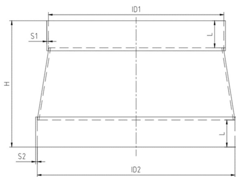
AGRU REDUCER
