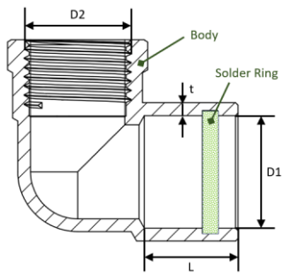
Sectional drawing
