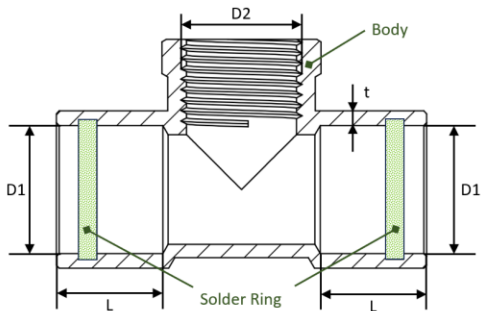
Sectional drawing
