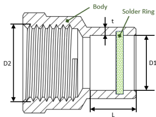
Sectional drawing
