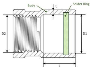
Sectional drawing
