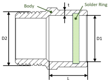
Sectional drawing
